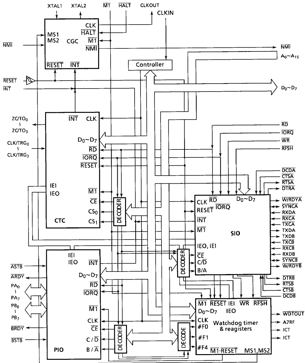
Figure 3.2.23 Block Diagram of the TMPZ84C015B Functioning As Evaluator
