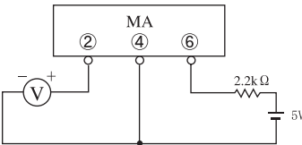
Fig1. Measurement Circuit
